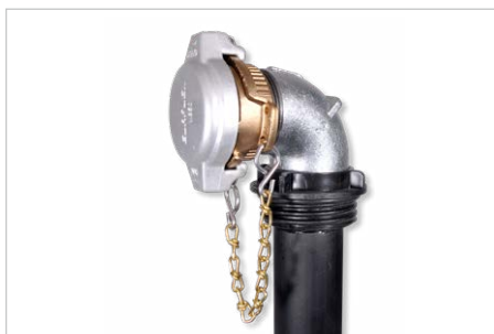
Suction connection for emptying by tanker lorry, for 700 litre tank, Order no. 117783 Suction connection for emptying by tanker lorry, for 1000 litre tank, Order no. 130199
