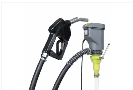
Electric pump with automatic nozzle, for diesel, Delivery rate: approx. 37 l/min, Order no. 117541
